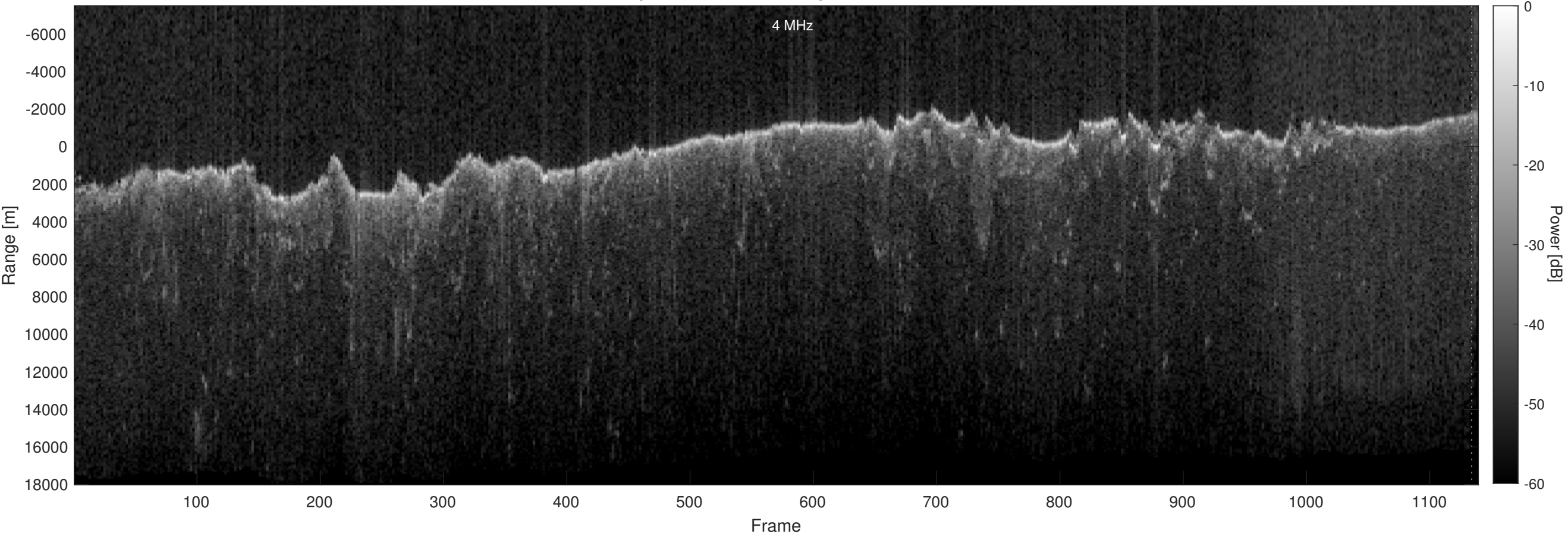
Orbit 15488, Optimized, Window, Depth-Corrected, Channel 2
