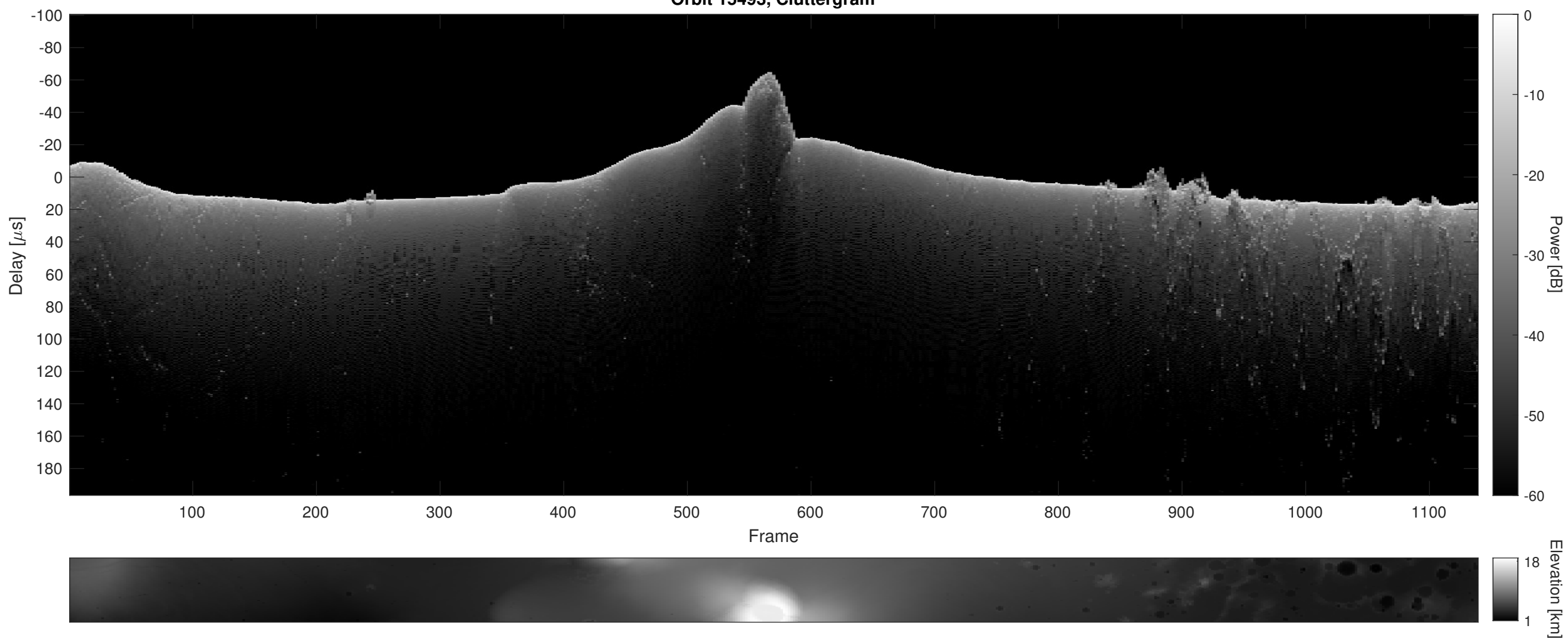
Orbit 15493, Cluttergram
