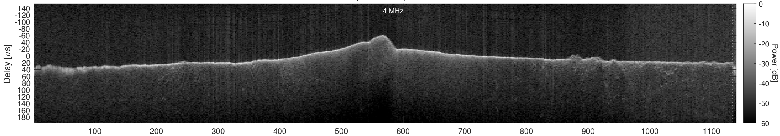
Orbit 15493, Window, Channel 1, Chapman
