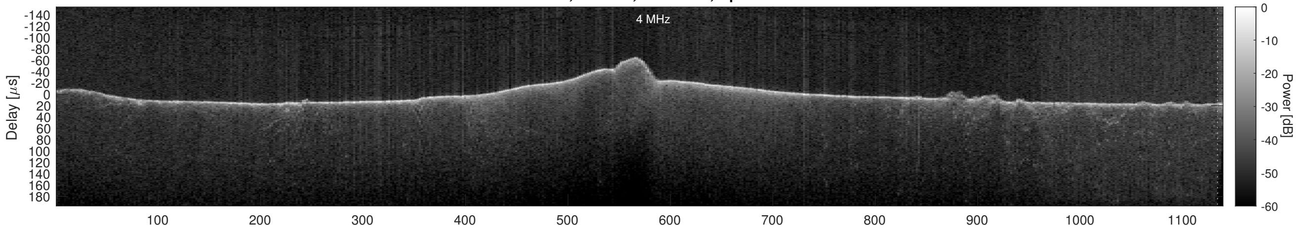
Orbit 15493, Cluttergram
