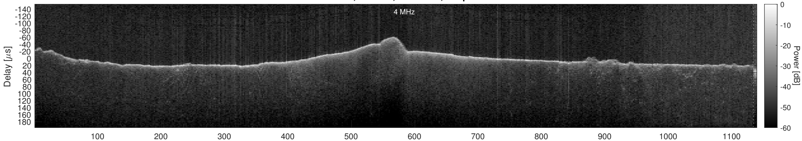
Orbit 15493, Window, Channel 1, Optimized
