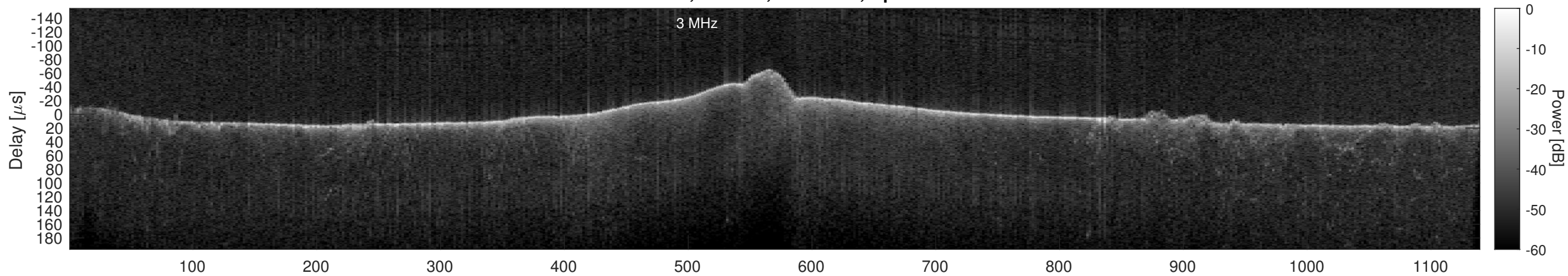
Orbit 15493, Cluttergram
