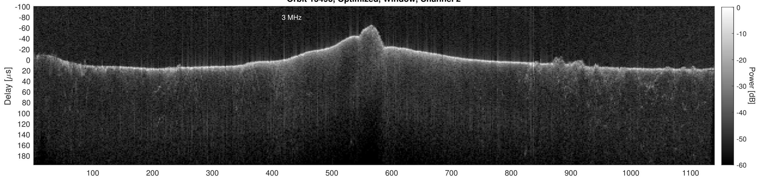
Orbit 15493, Cluttergram
