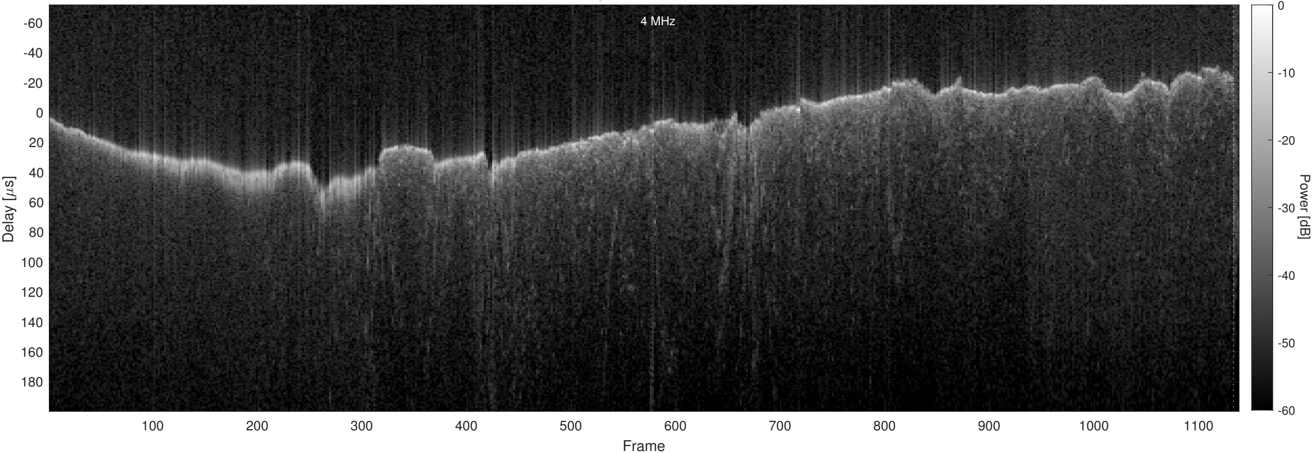
Orbit 15497, Chapman, No Window, Channel 2
