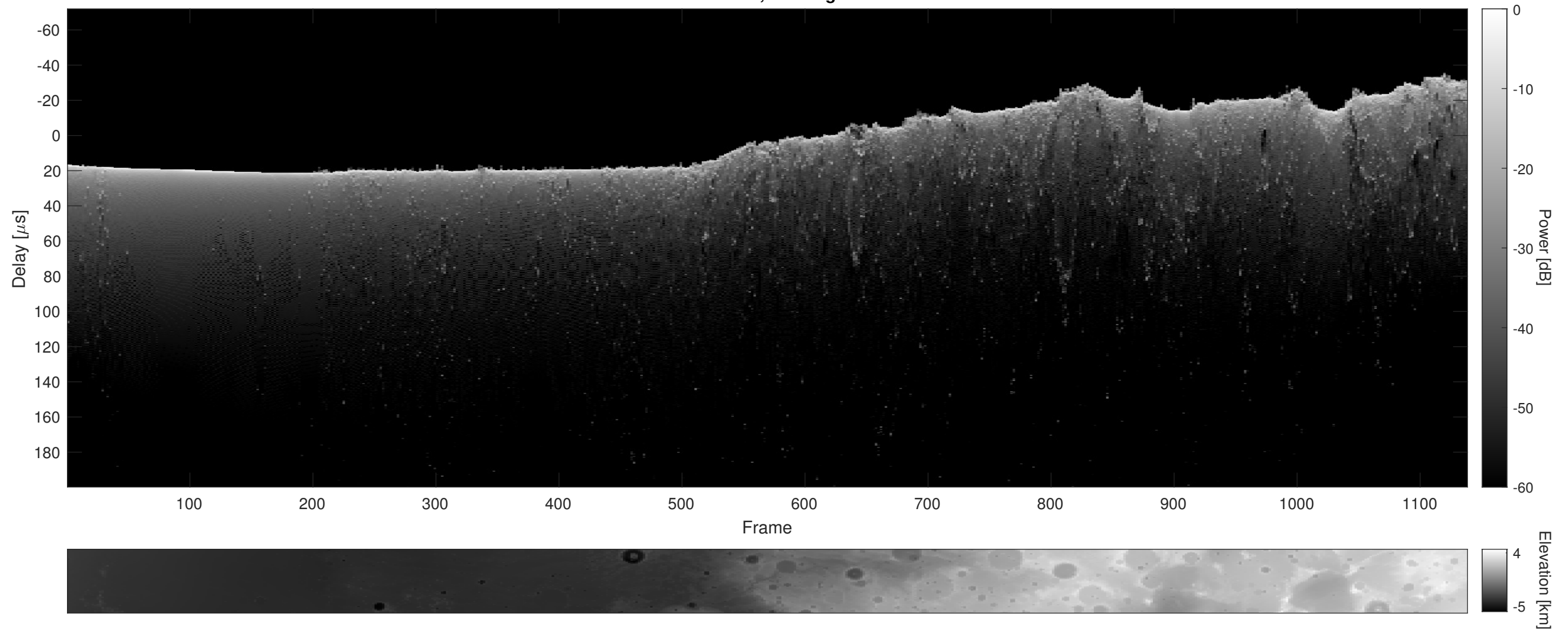
Orbit 15497, Cluttergram
