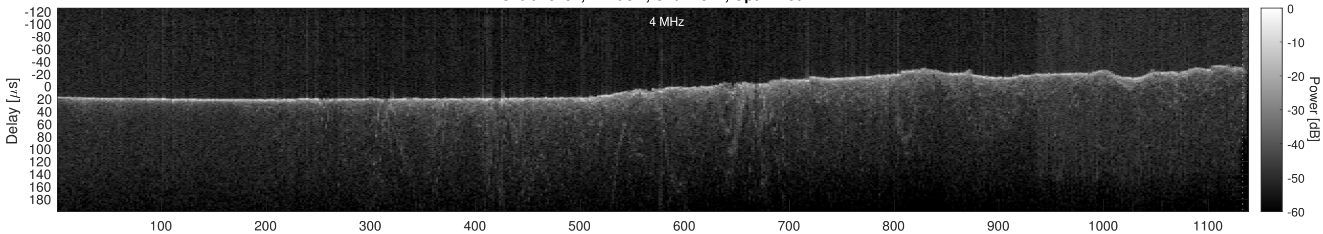
Orbit 15497, Cluttergram
