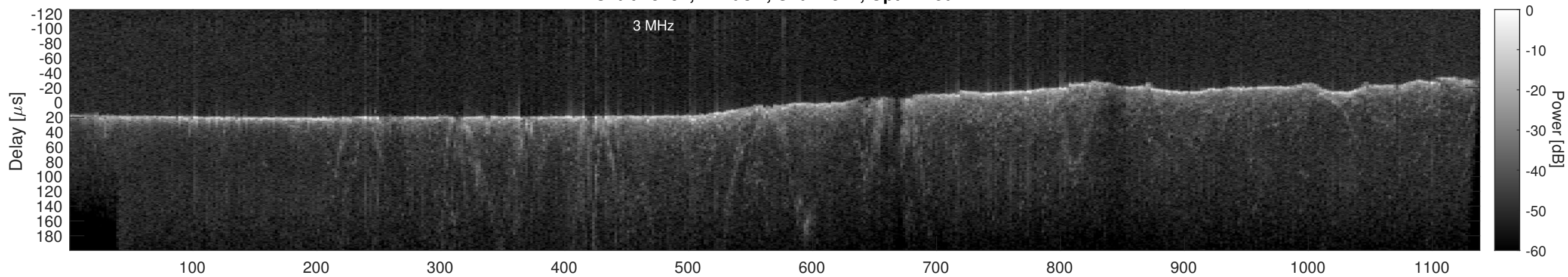
Orbit 15497, Cluttergram
