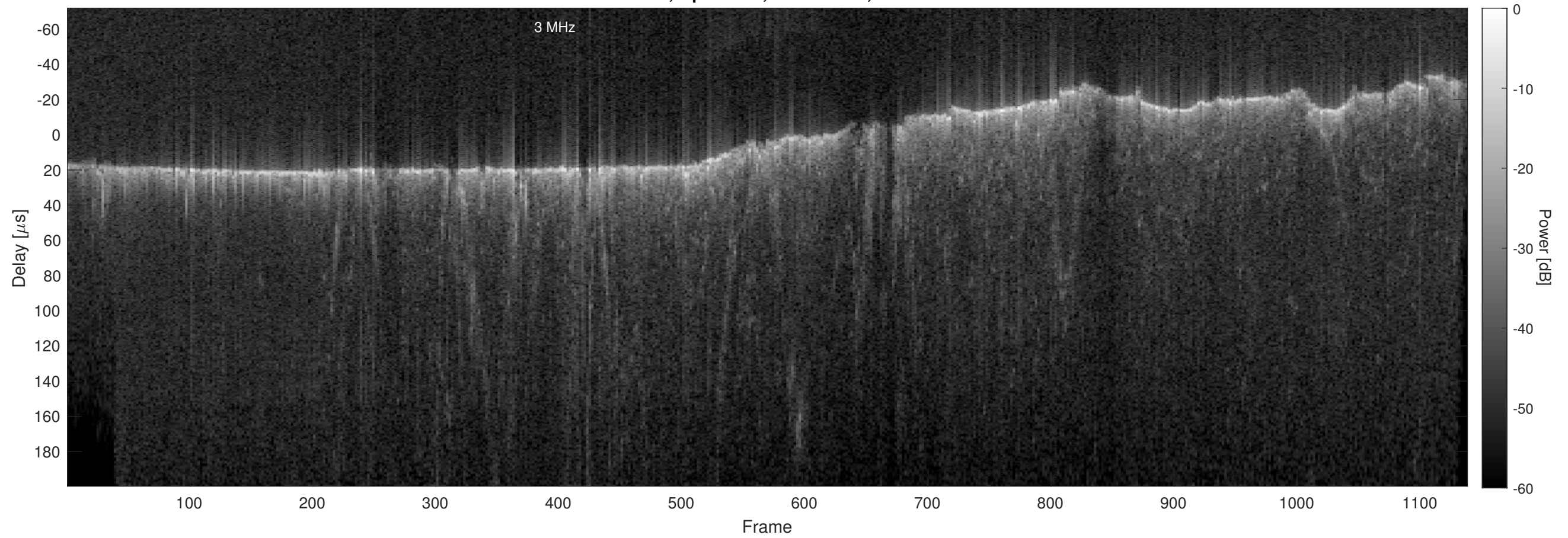
Orbit 15497, Optimized, No Window, Channel 2
