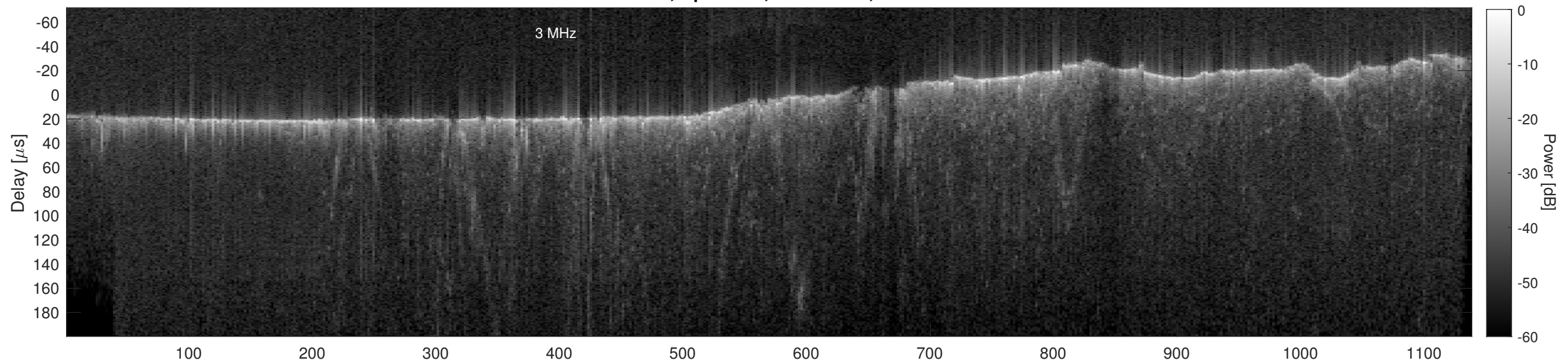
Orbit 15497, Cluttergram
