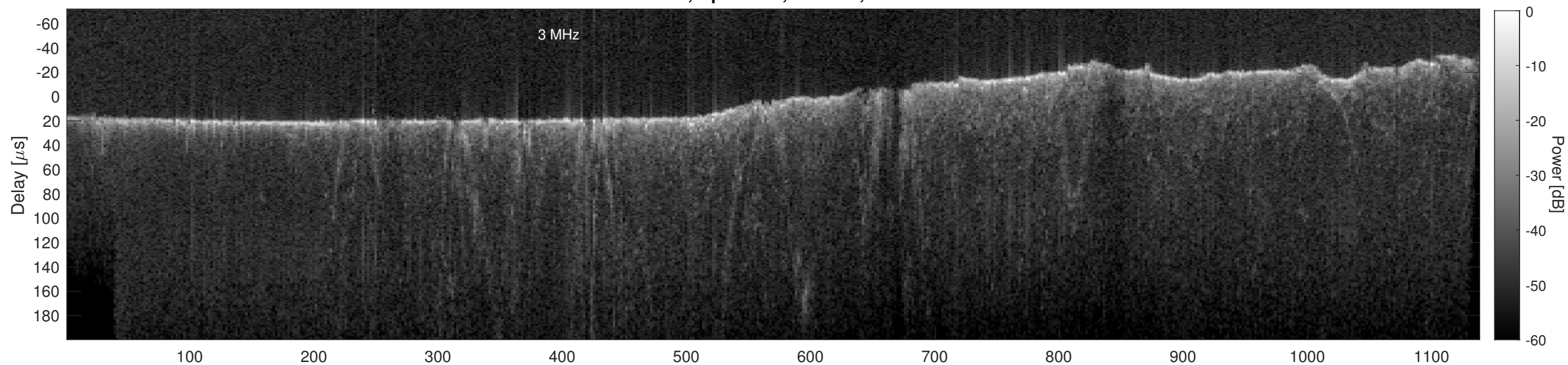
Orbit 15497, Cluttergram
