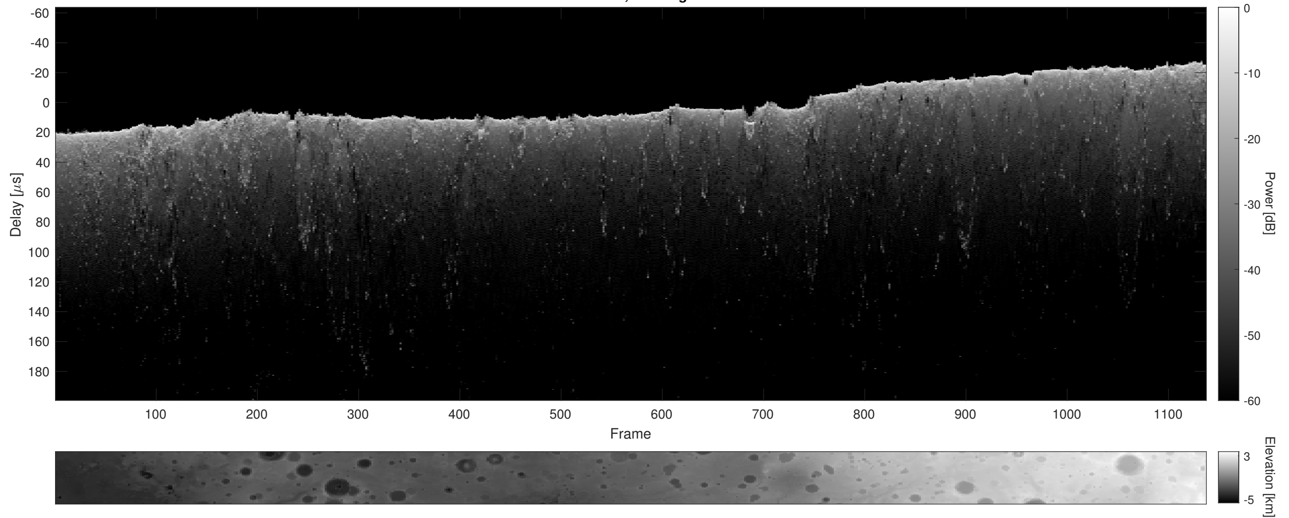
Orbit 15499, Cluttergram
