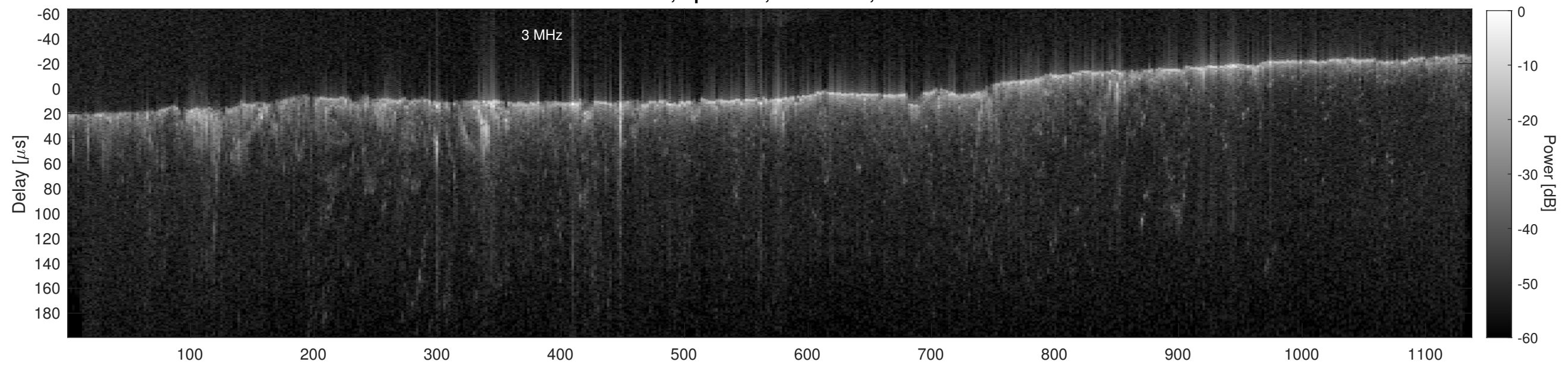
Orbit 15499, Cluttergram
