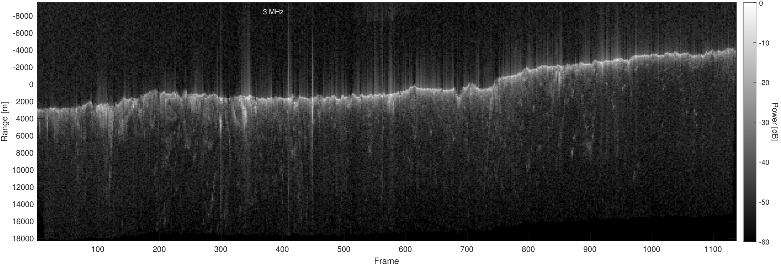
Orbit 15499, Optimized, No Window, Depth-Corrected, Channel 2
