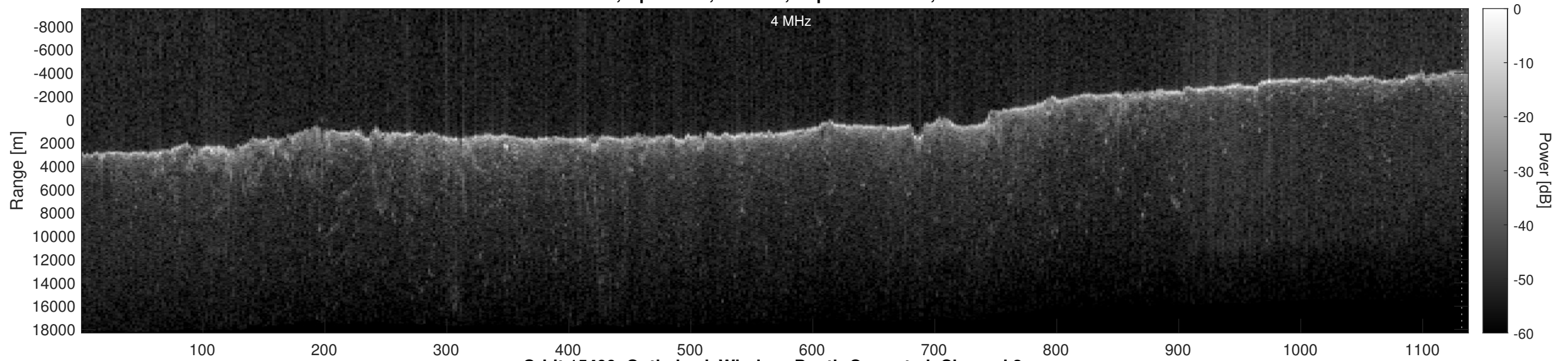
Orbit 15499, Optimized, Window, Depth-Corrected, Channel 2
