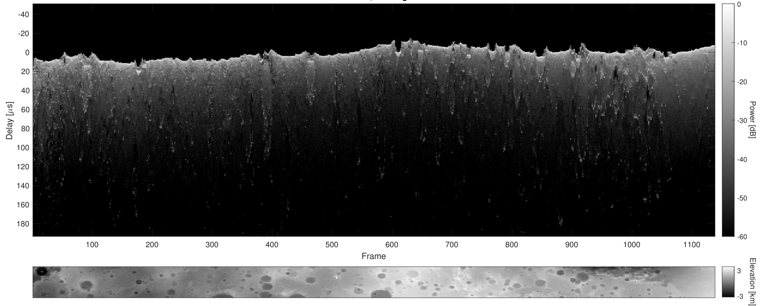
Orbit 15502, Cluttergram
