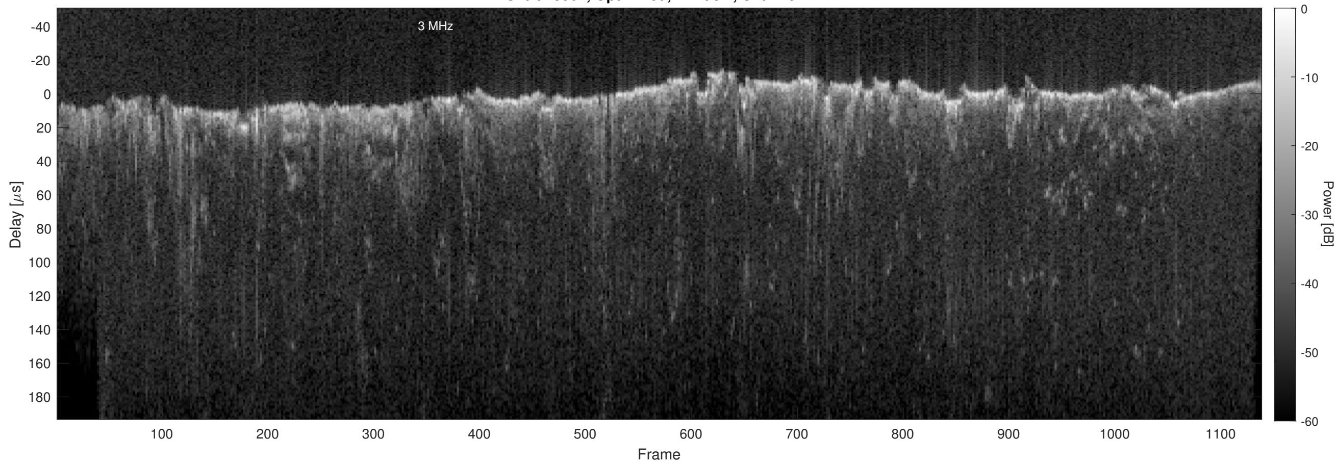
Orbit 15502, Optimized, Window, Channel 2
