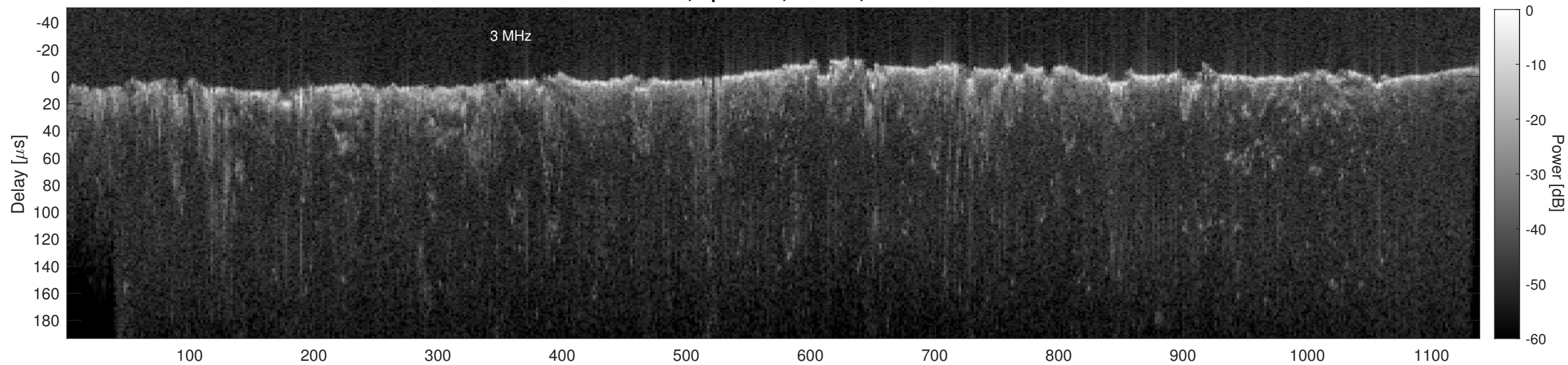
Orbit 15502, Cluttergram
