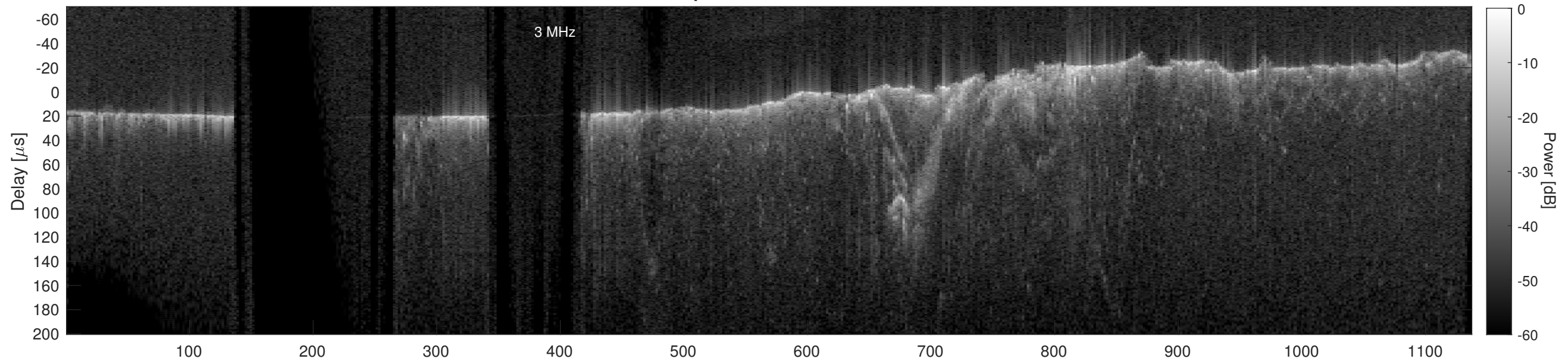
Orbit 15504, Cluttergram
