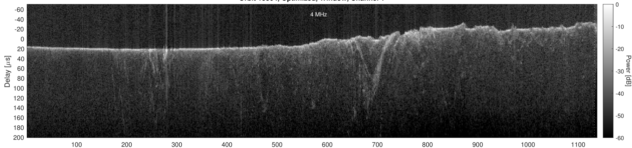
Orbit 15504, Optimized, Window, Channel 2
