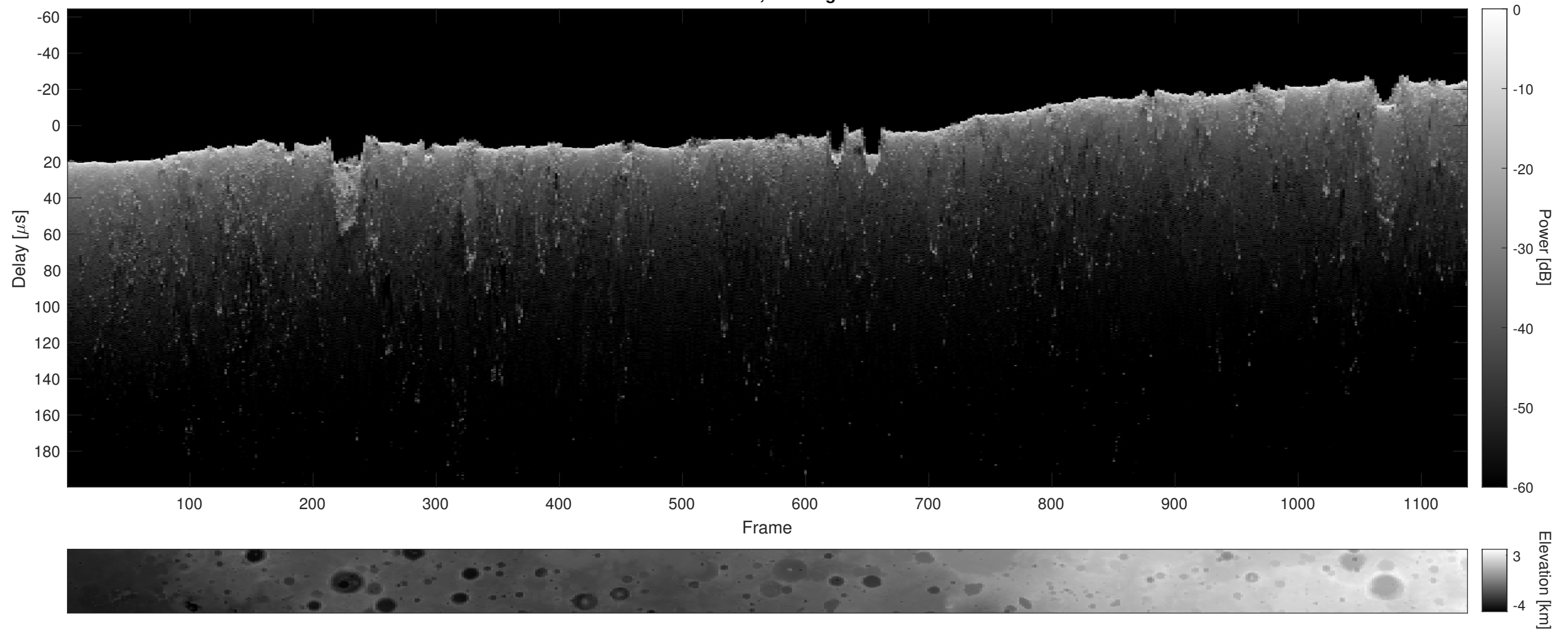
Orbit 15506, Cluttergram
