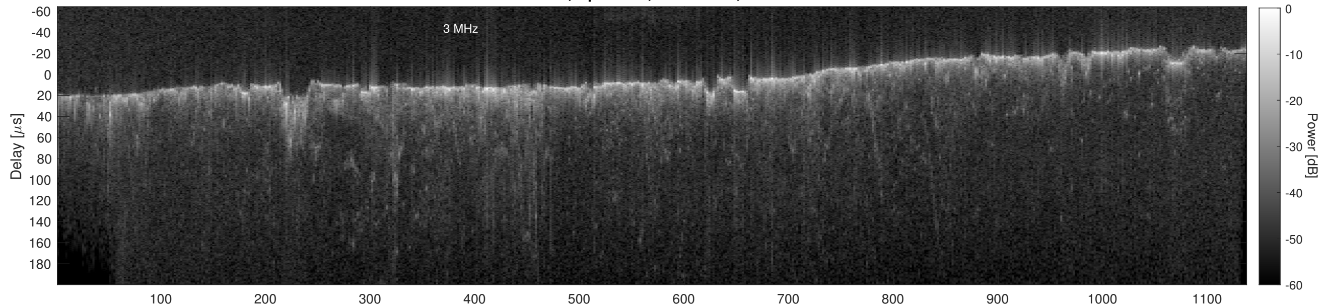
Orbit 15506, Cluttergram
