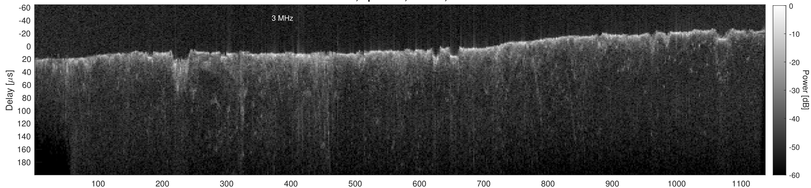
Orbit 15506, Cluttergram
