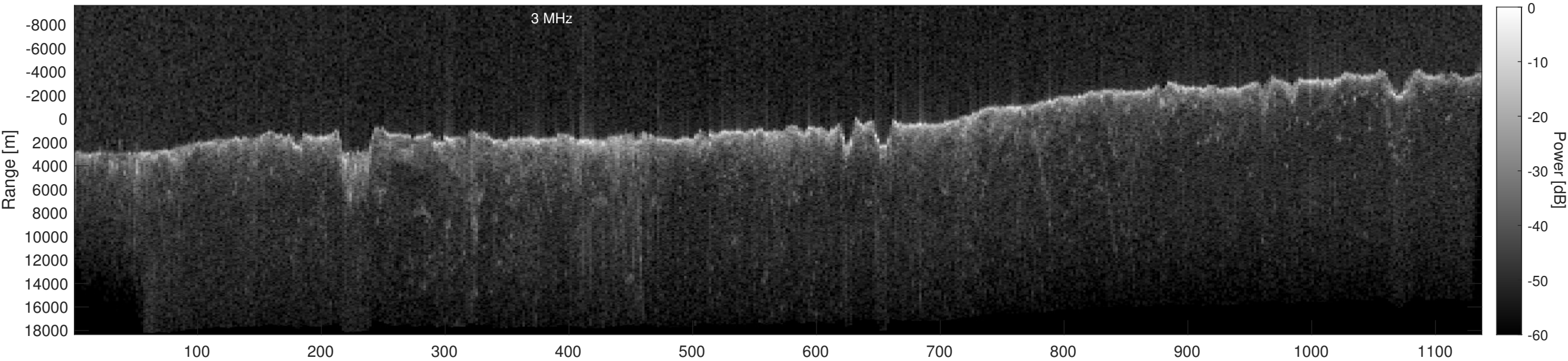
Orbit 15506, Depth-Corrected Cluttergram
