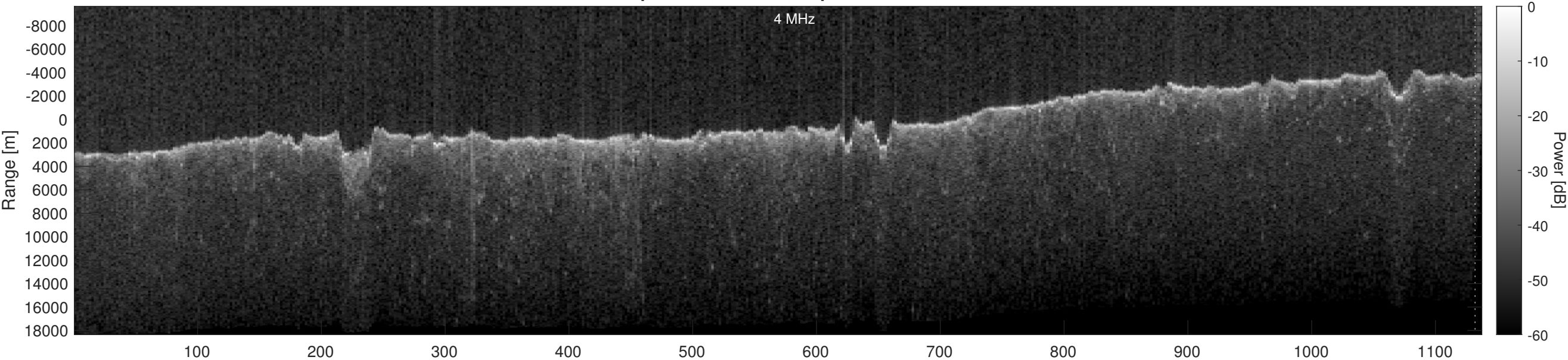
Orbit 15506, Optimized, Window, Depth-Corrected, Channel 2
