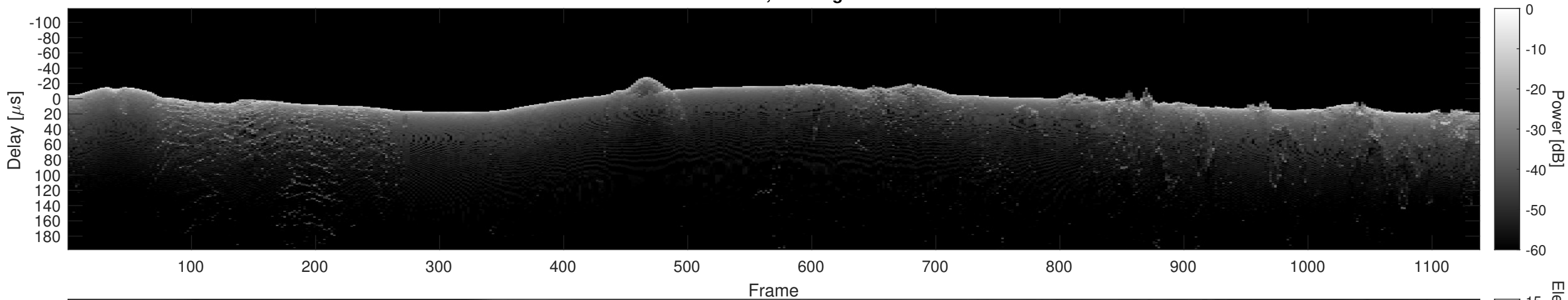
Orbit 15507, Cluttergram
