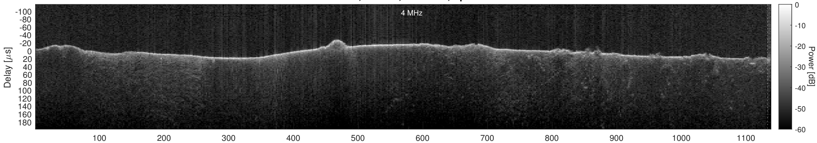
Orbit 15507, Cluttergram
