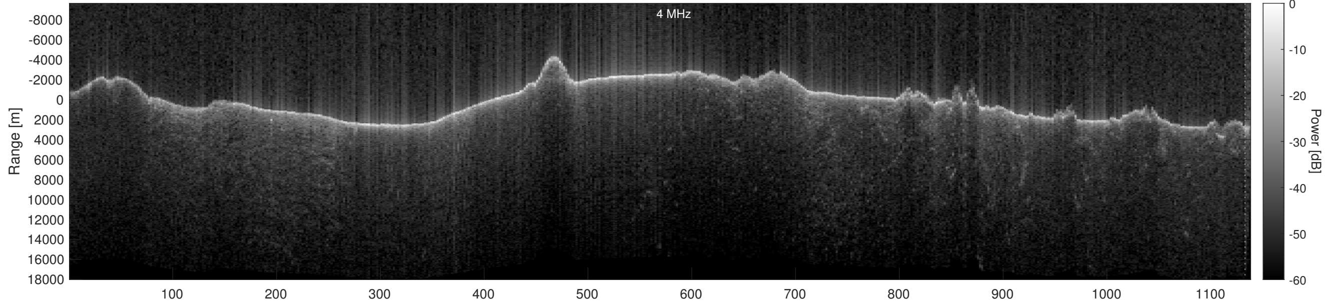
Orbit 15507, Optimized, No Window, Depth-Corrected, Channel 2
