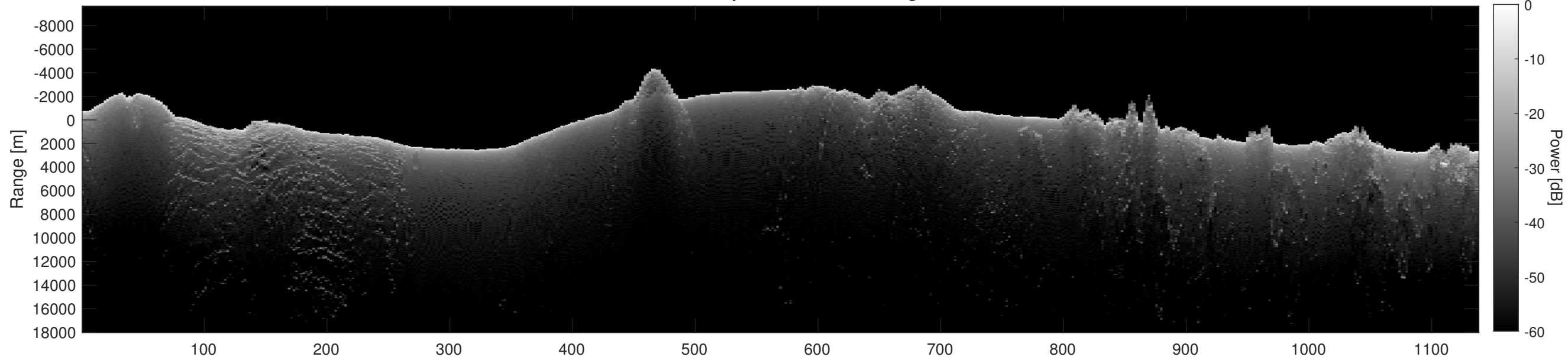
Orbit 15507, Depth-Corrected Cluttergram
