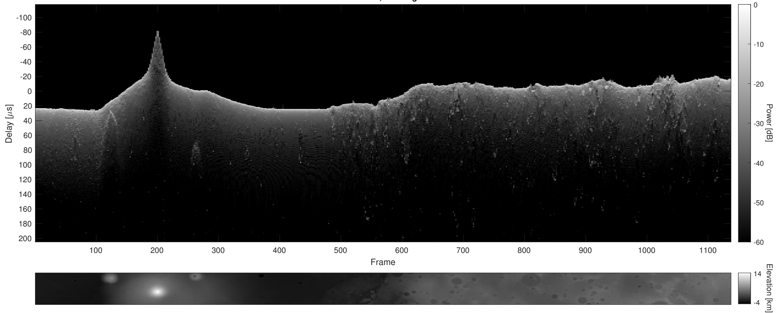
Orbit 15508, Cluttergram
