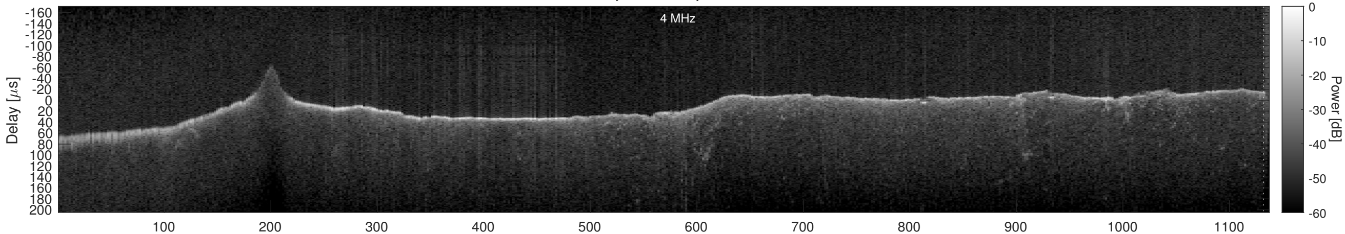
Orbit 15508, Window, Channel 1, Chapman
