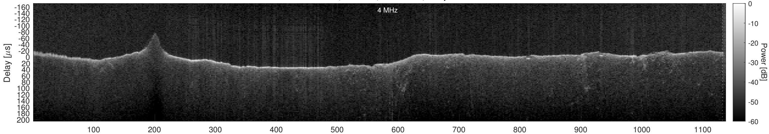
Orbit 15508, Window, Channel 1, Optimized
