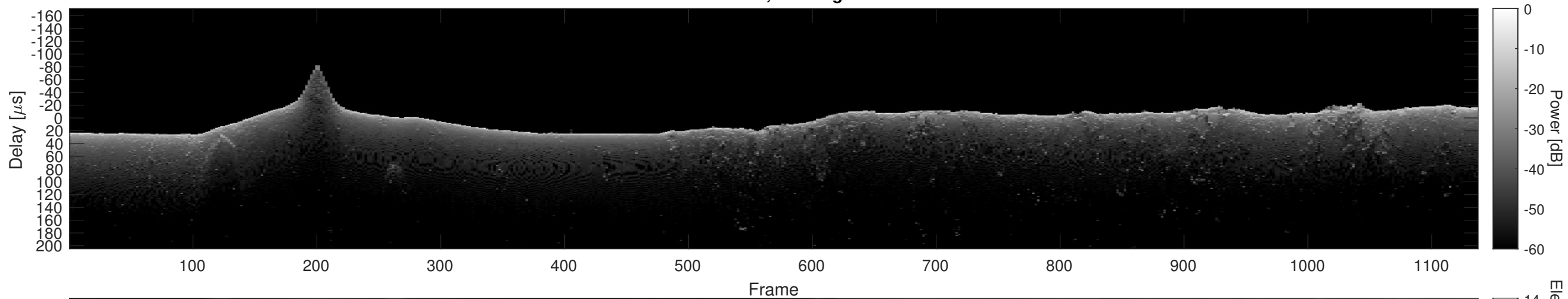
Orbit 15508, Cluttergram
