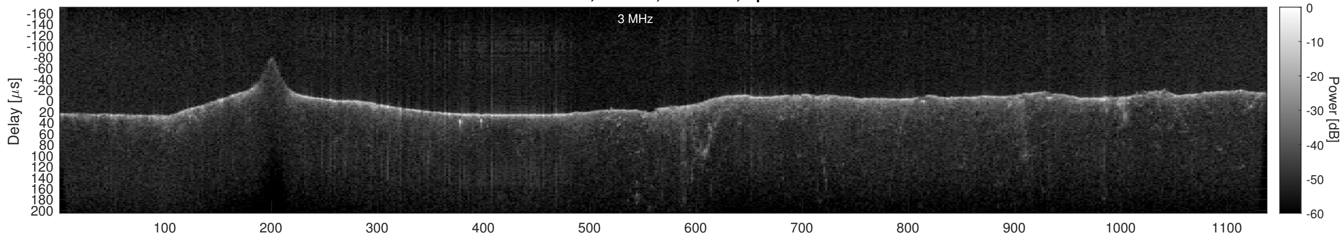
Orbit 15508, Cluttergram
