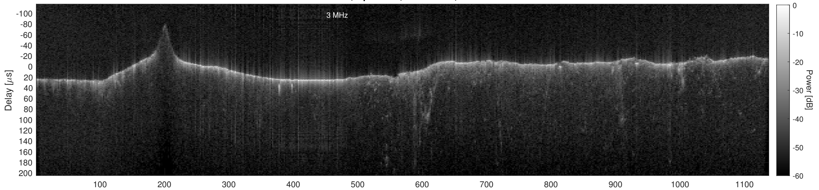
Orbit 15508, Cluttergram
