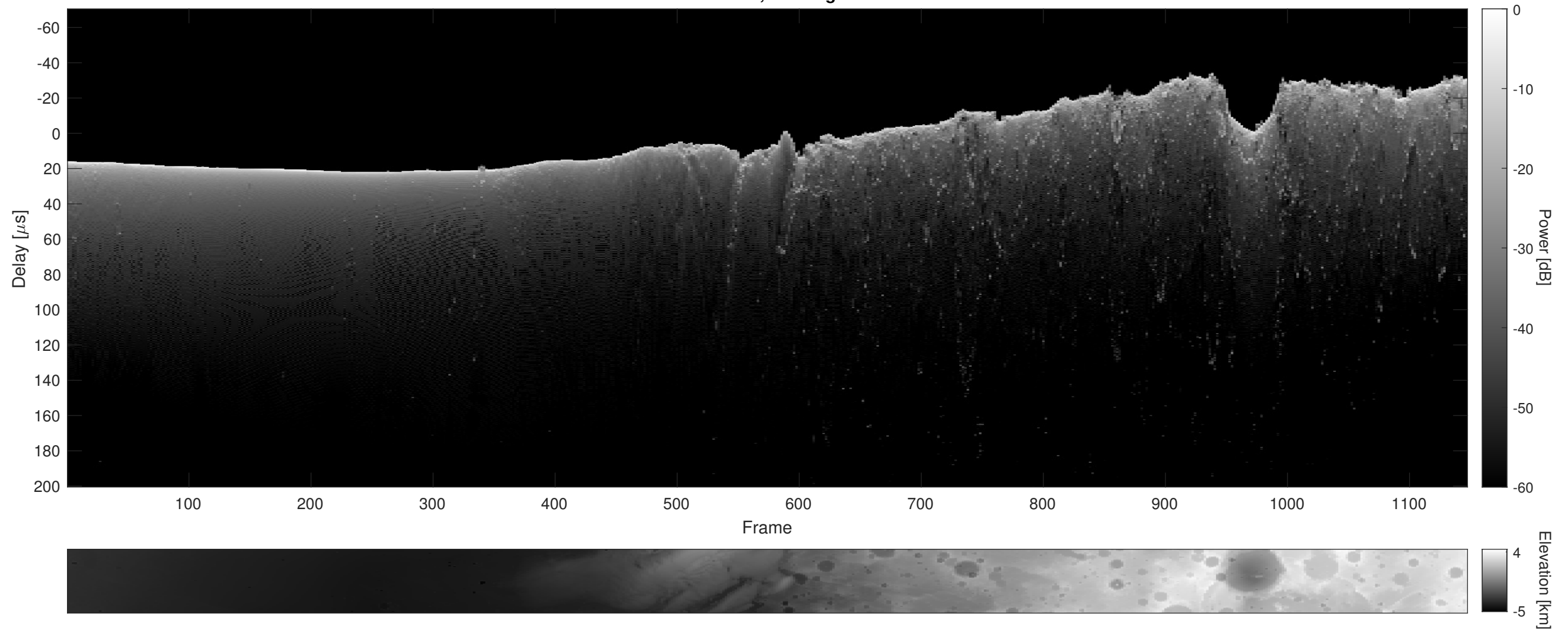
Orbit 15511, Cluttergram
