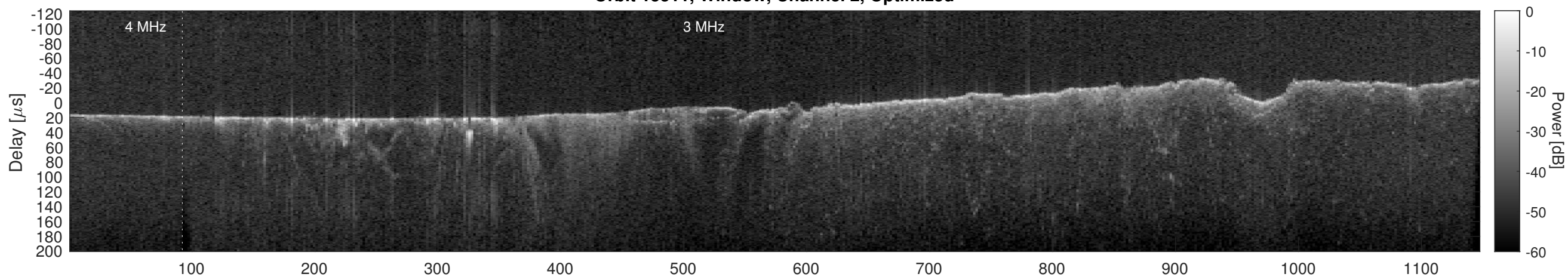
Orbit 15511, Cluttergram
