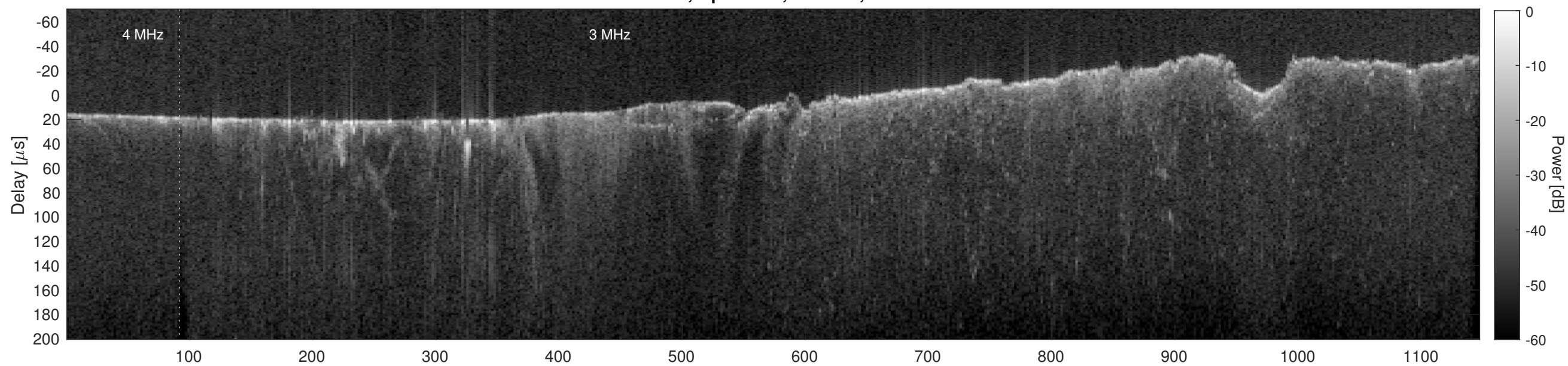
Orbit 15511, Cluttergram
