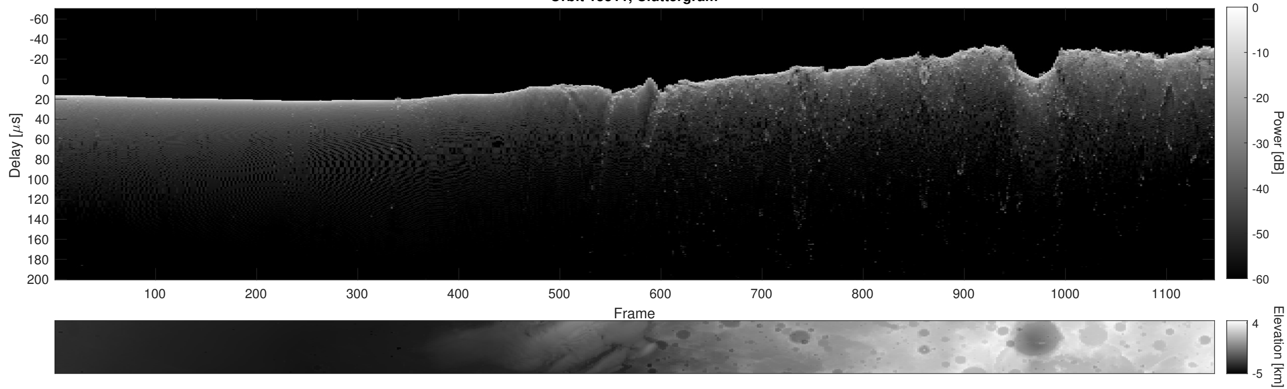
Orbit 15511, Cluttergram
