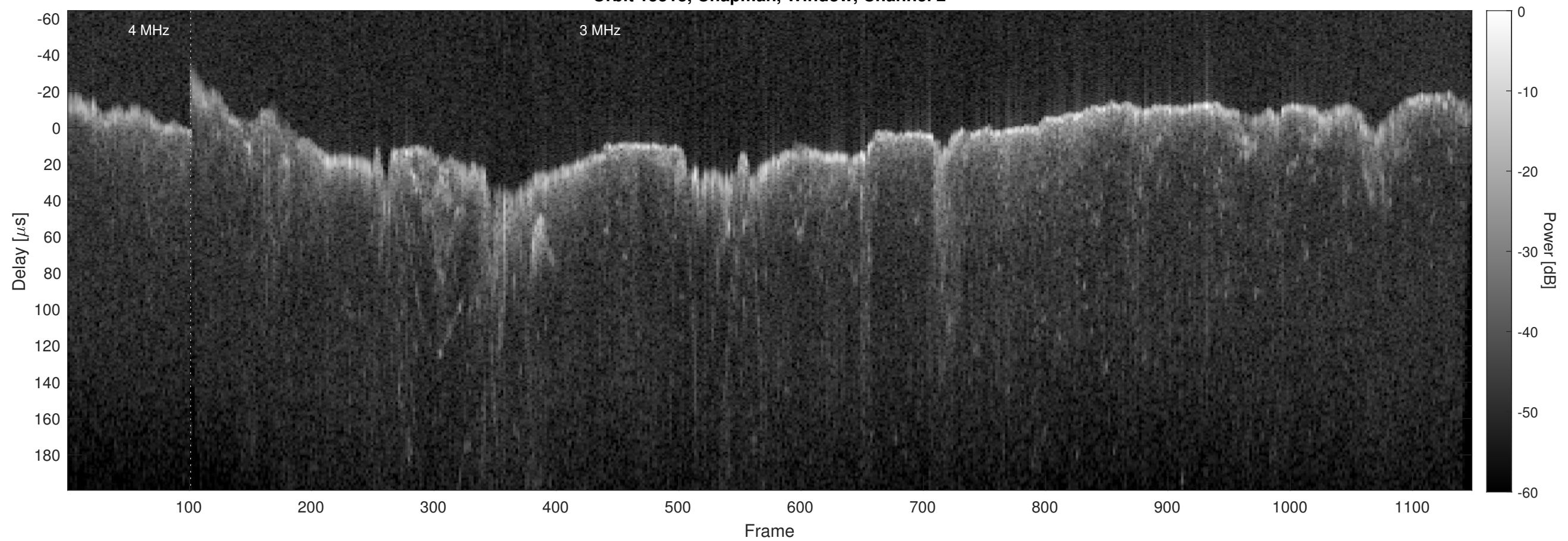
Orbit 15513, Chapman, Window, Channel 2
