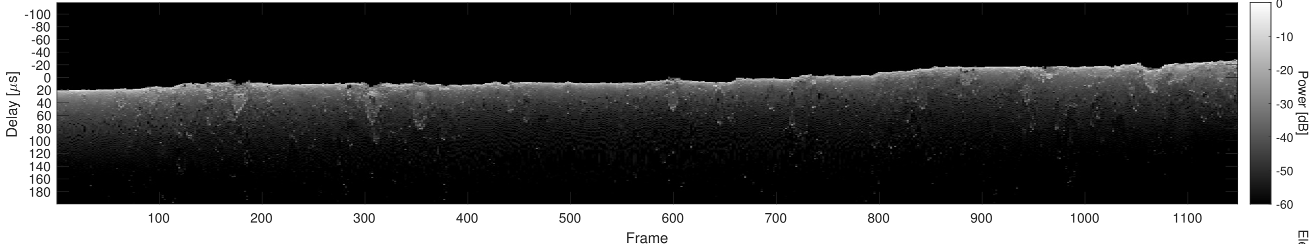
Orbit 15513, Cluttergram
