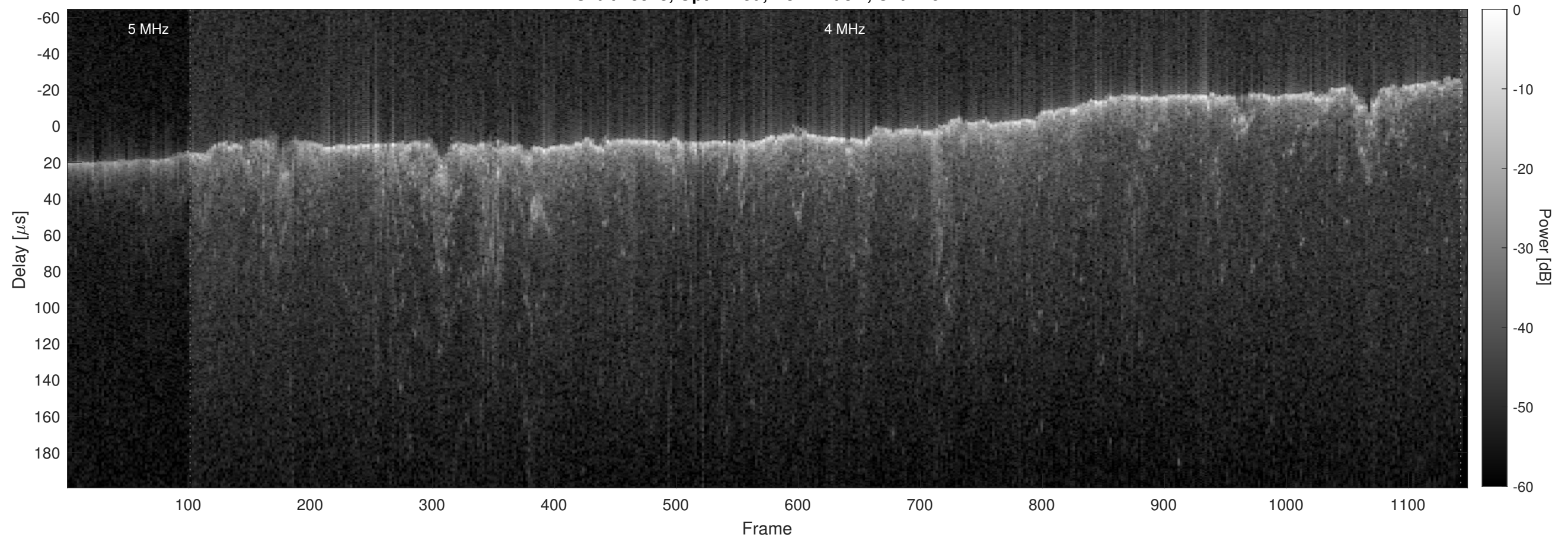
Orbit 15513, Optimized, No Window, Channel 2
