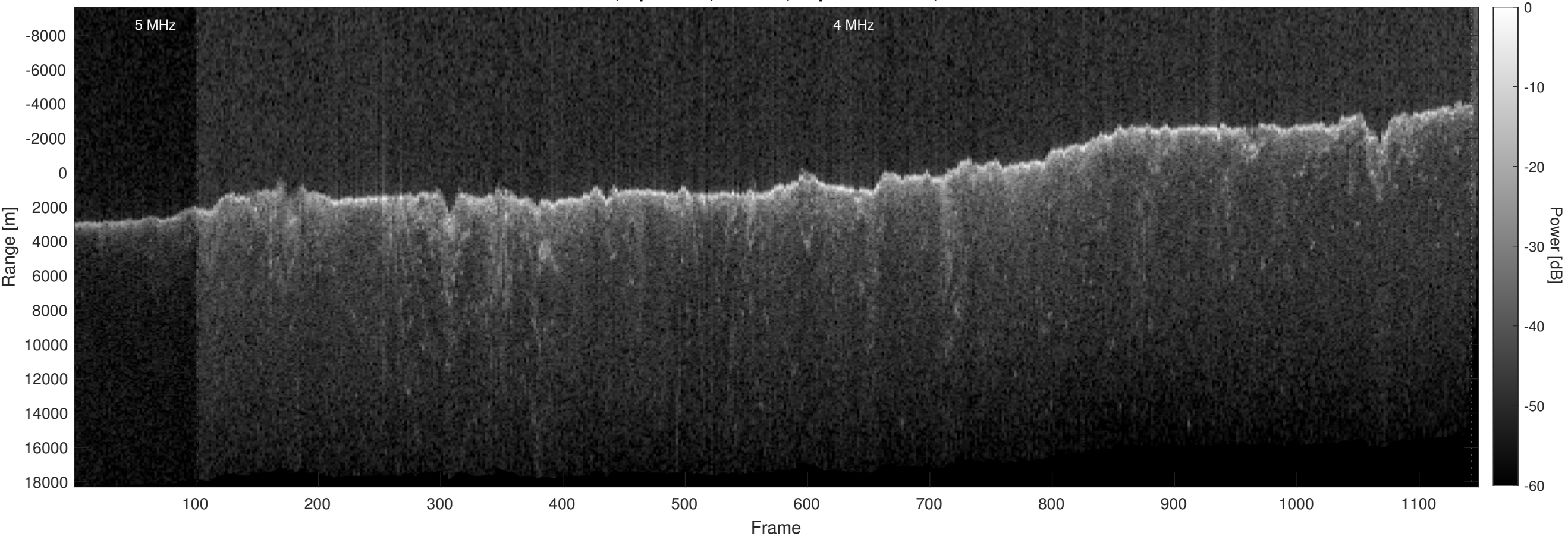
Orbit 15513, Optimized, Window, Depth-Corrected, Channel 2
