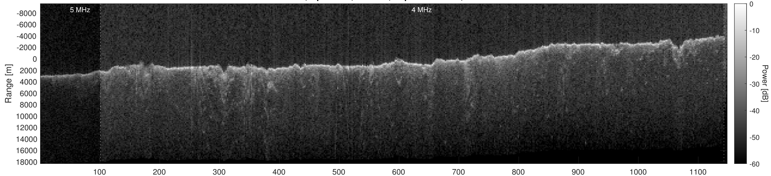
Orbit 15513, Optimized, Window, Depth-Corrected, Channel 2
