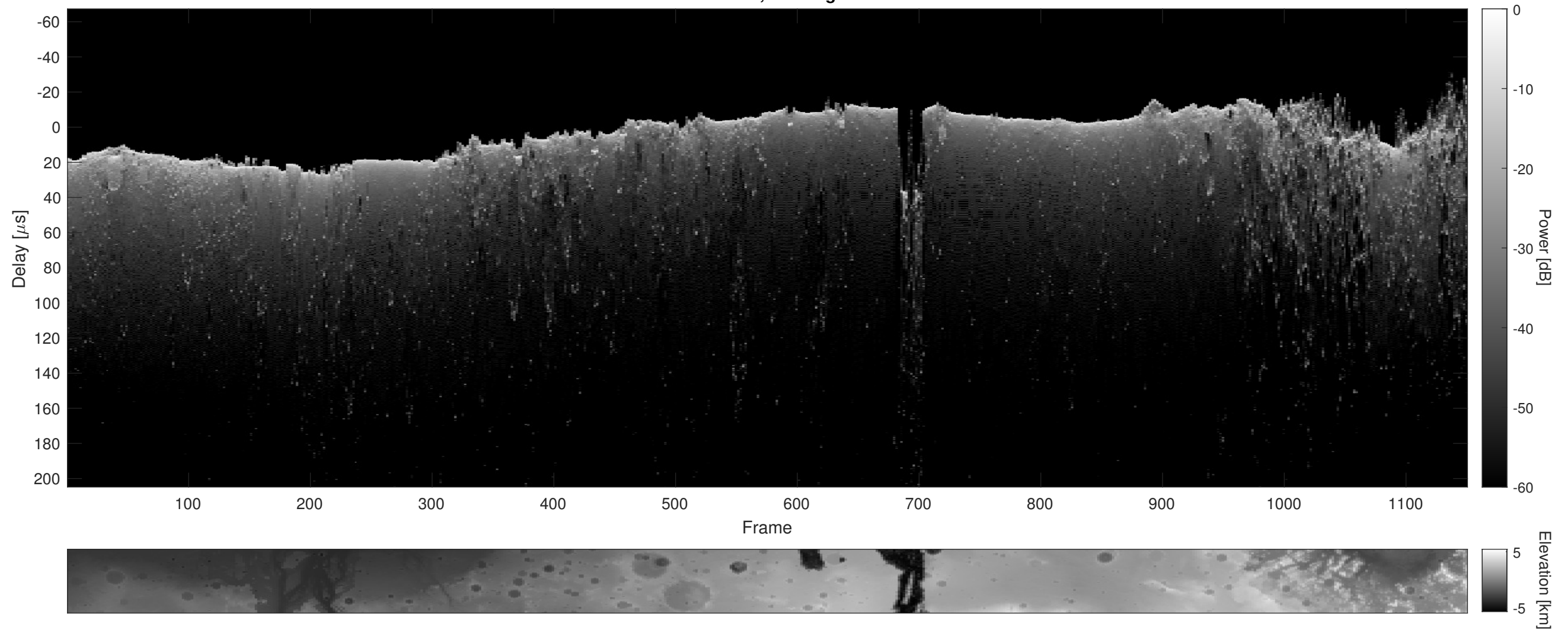
Orbit 15517, Cluttergram
