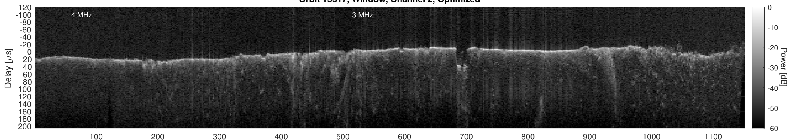
Orbit 15517, Cluttergram
