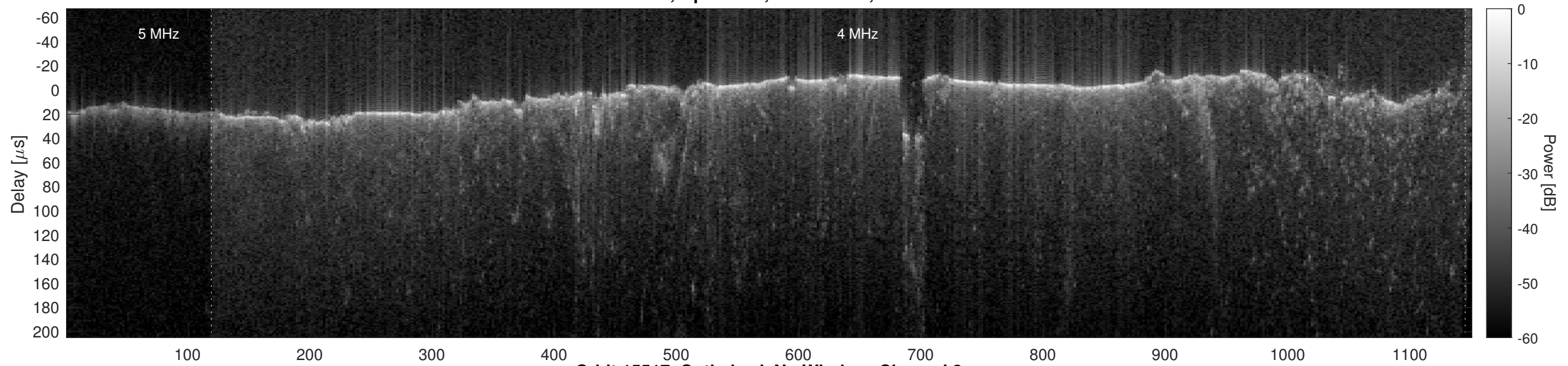
Orbit 15517, Optimized, No Window, Channel 2
