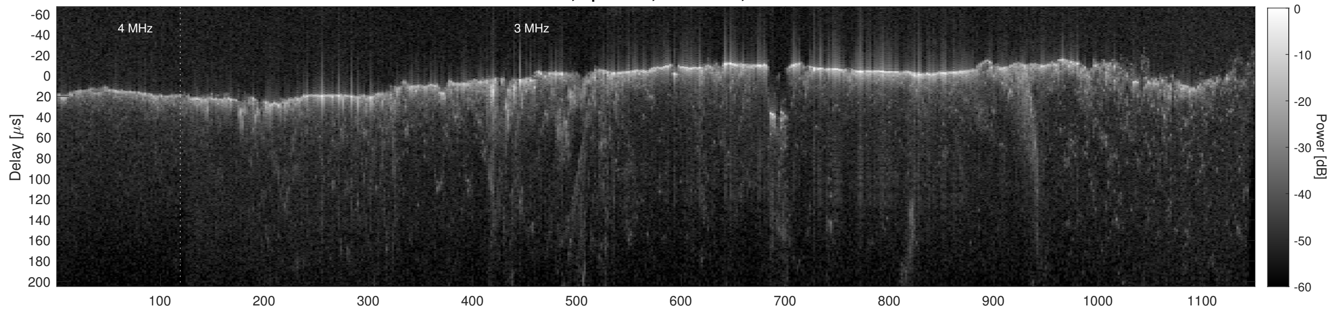
Orbit 15517, Cluttergram
