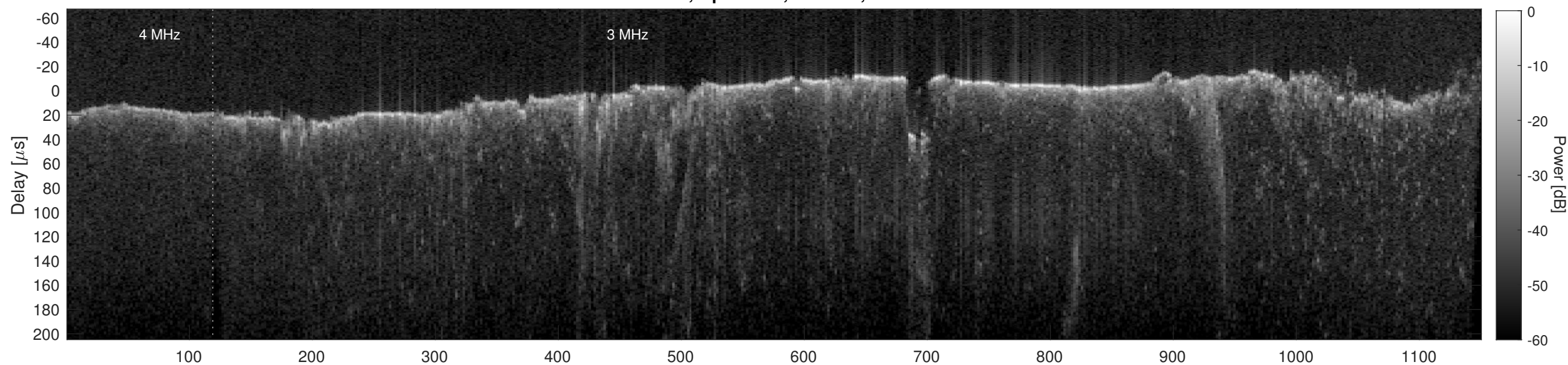
Orbit 15517, Cluttergram
