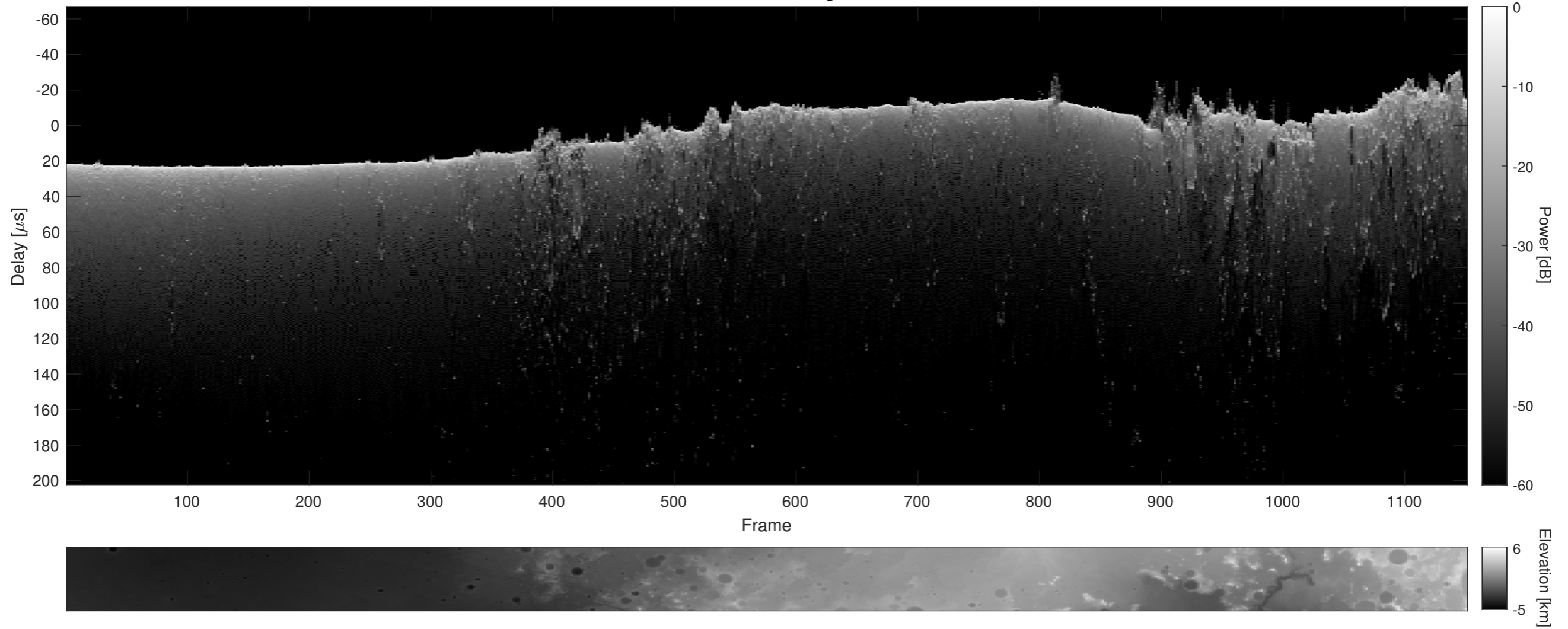
Orbit 15519, Cluttergram
