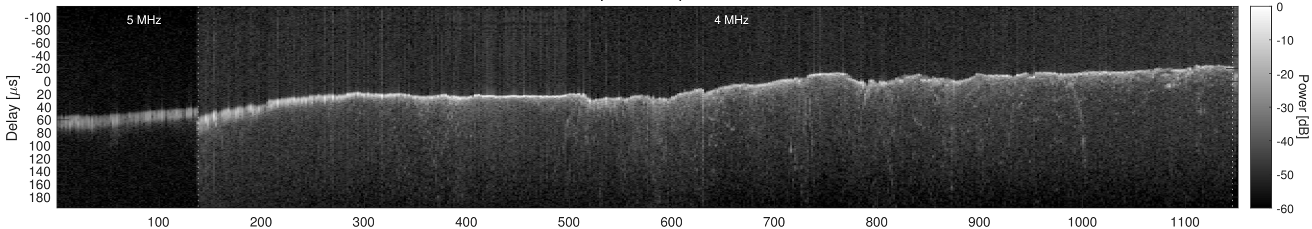
Orbit 15522, Window, Channel 1, Chapman
