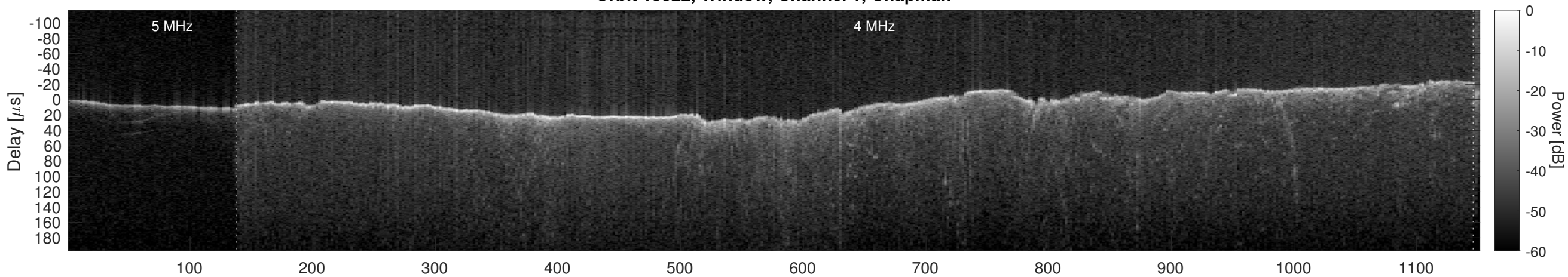
Orbit 15522, Window, Channel 1, Optimized
