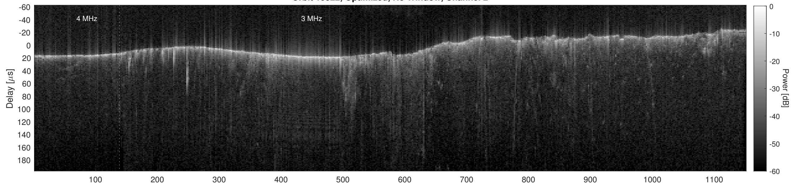
Orbit 15522, Cluttergram
