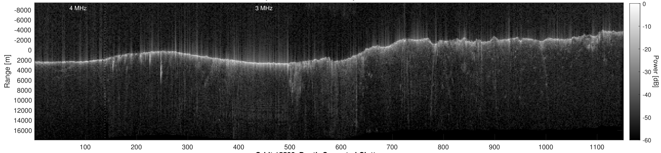
Orbit 15522, Depth-Corrected Cluttergram
