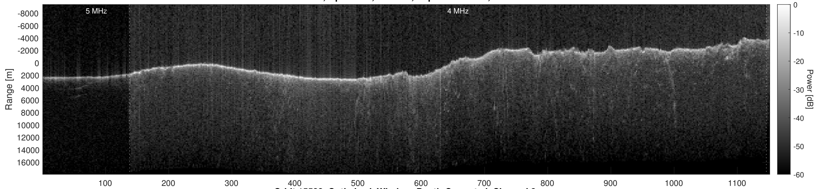
Orbit 15522, Optimized, Window, Depth-Corrected, Channel 2
