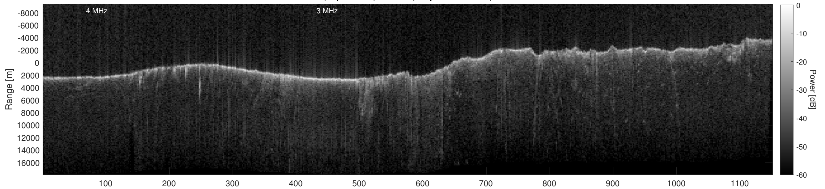
Orbit 15522, Depth-Corrected Cluttergram
