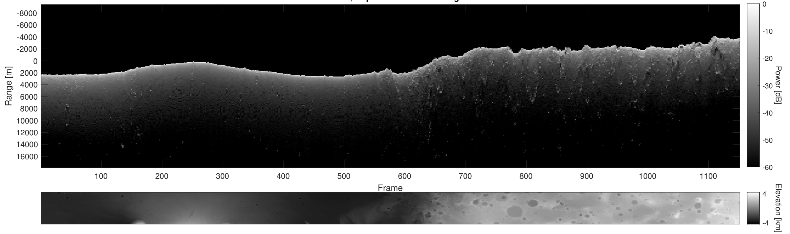
Orbit 15522, Depth-Corrected Cluttergram
