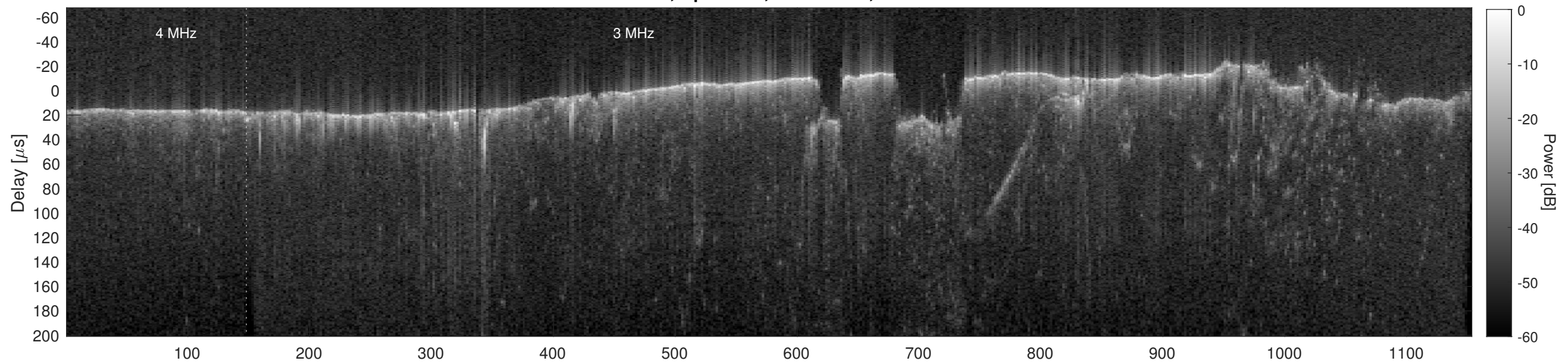
Orbit 15524, Cluttergram
