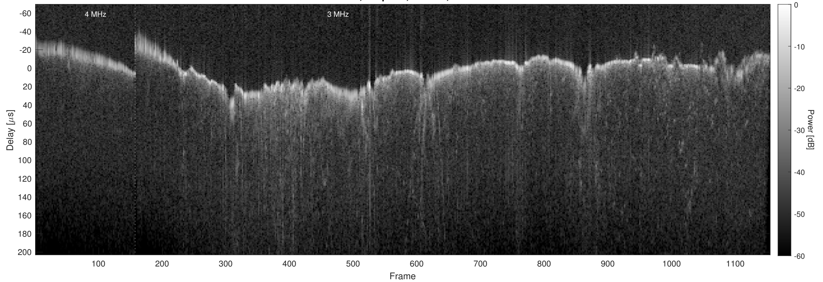
Orbit 15526, Chapman, Window, Channel 2
